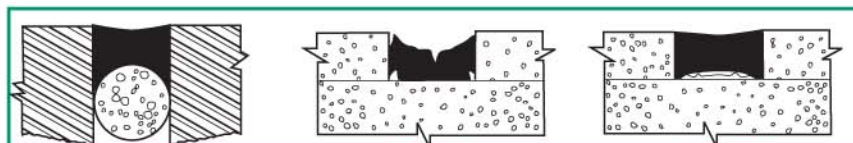
FIGURE 1 Proper Depth Control The effects on the sealant with and without bond breakers are illustrated in Figures Two and Three. FIGURE 2 Joints without Bond Breaker FIGURE 3 Joints with Bond Breaker
